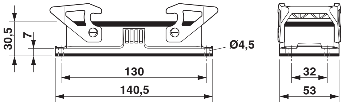
Dimensional drawing
