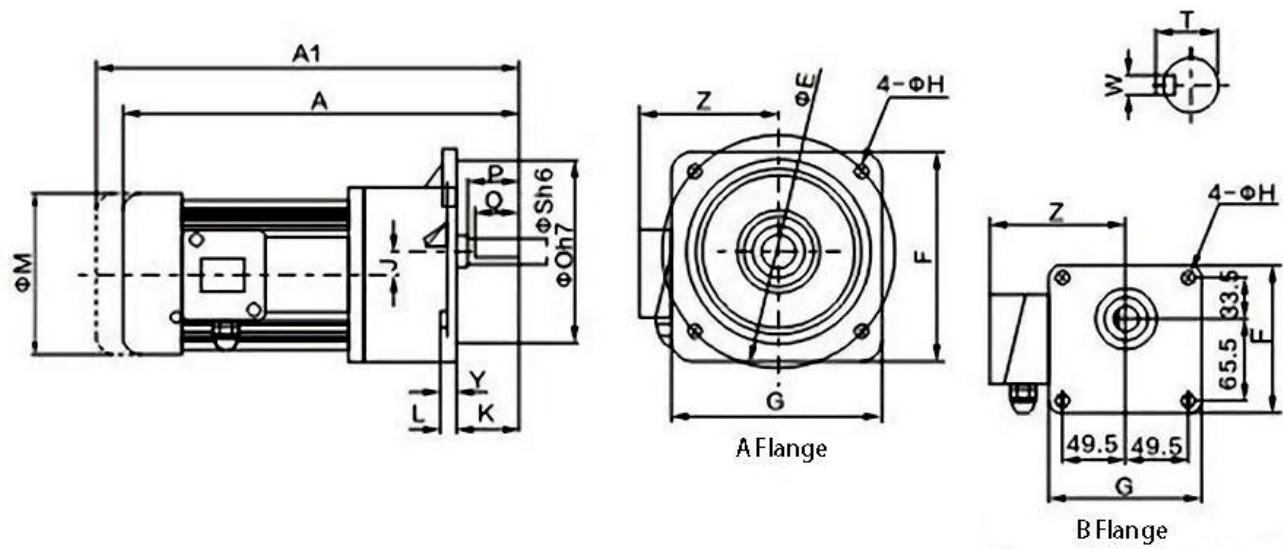
100W Vertical AC Gear Motor Dimensions (Unit: mm)
