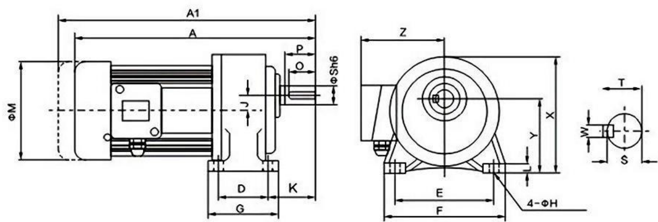
100W Horizontal AC Gear Motor Dimensions (Unit: mm)
