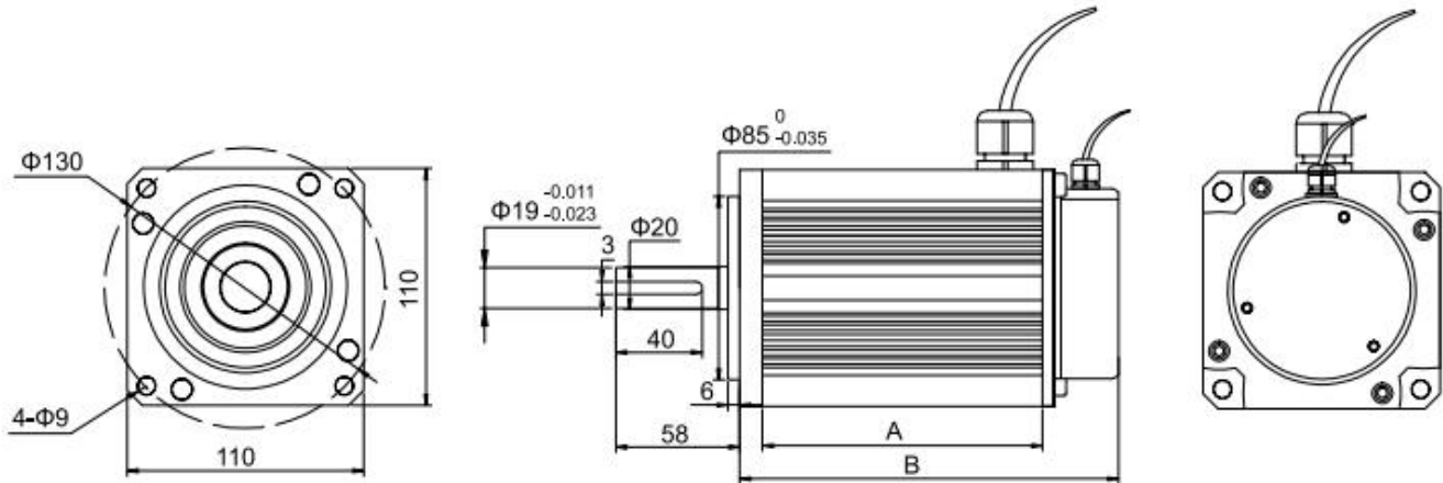
DIMENSION: UNIT=mm
