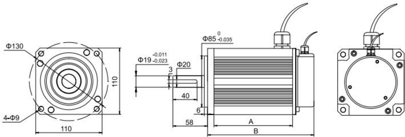
DIMENSION: UNIT=mm
