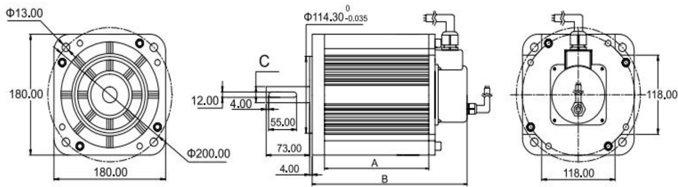
DIMENSION: UNIT=mm
