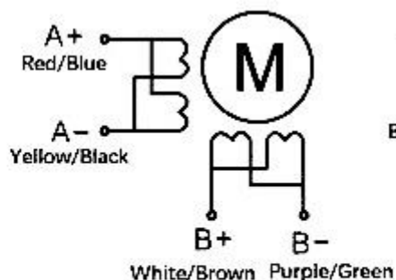
Parallel connection (for high speed)
